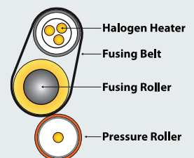
State-of-the-art belt fusing system consumes less power and shortens warm-up time.
