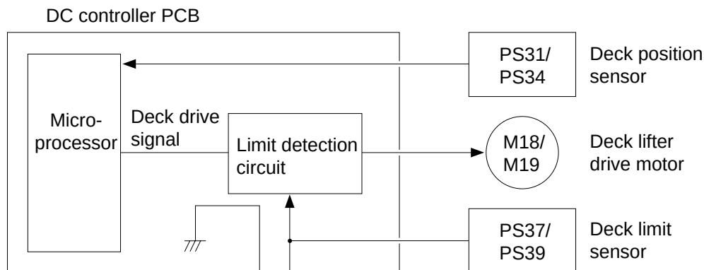
Figure 5-306 Deck Limit Detection (2 cassettes + left/right deck)
