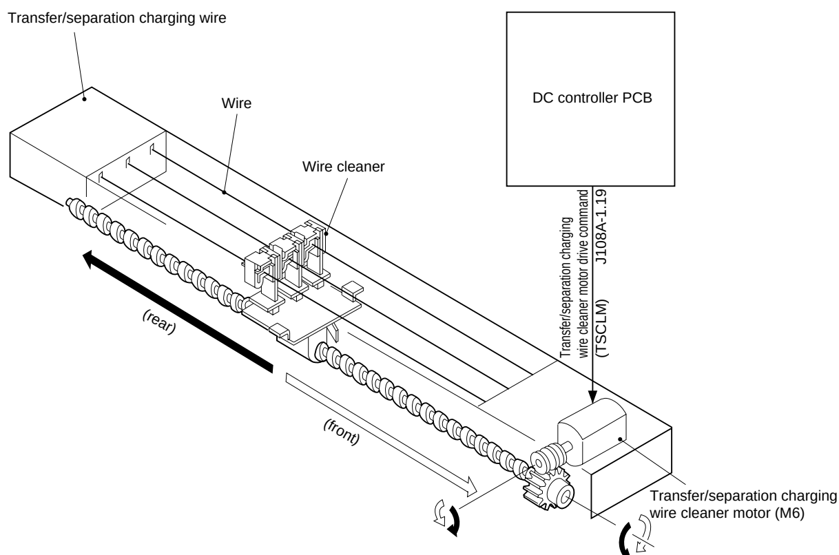
Figure 4-125 (transfer/separation charging assembly)
