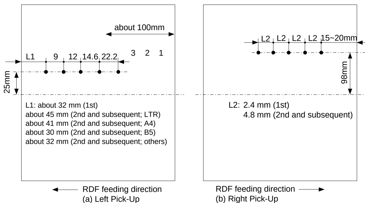
Figure 4-109 Points of Measurement on an Original
