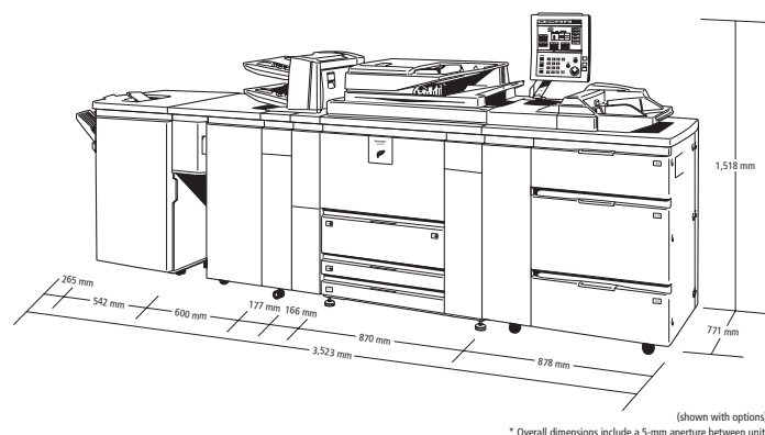
(shown with options) * Overall dimensions include a 5-mm aperture between units.
